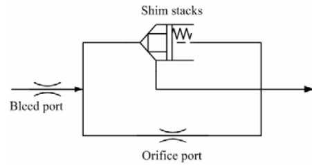
Fig. 3. The arrangement of the entire flow path in the piston assembly.
